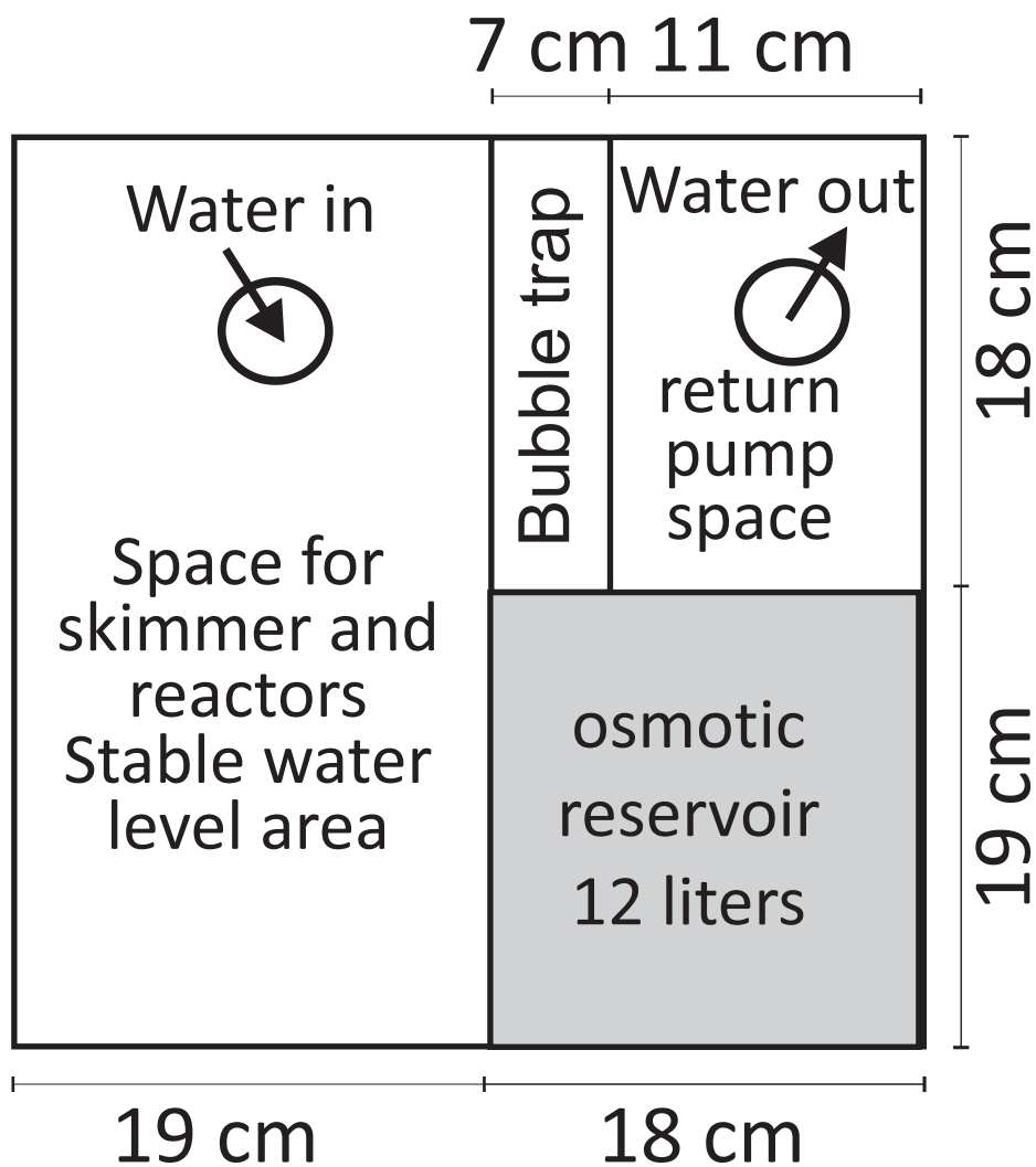
Ready Sump 38 top view
